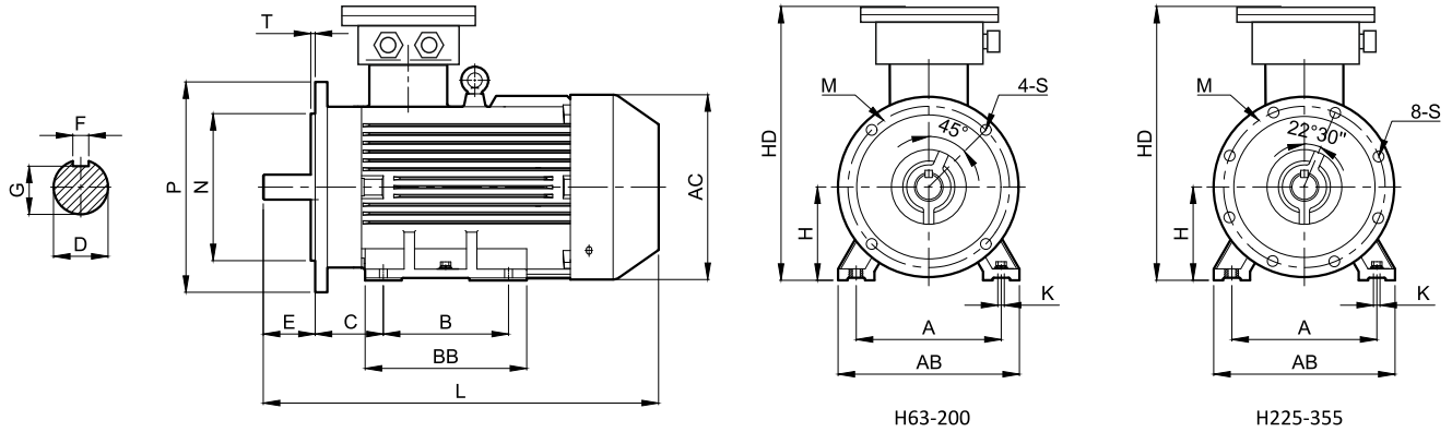
Mounting and overall dimensions Frame with feet, end-shield with flange (with through holes) (B35)
