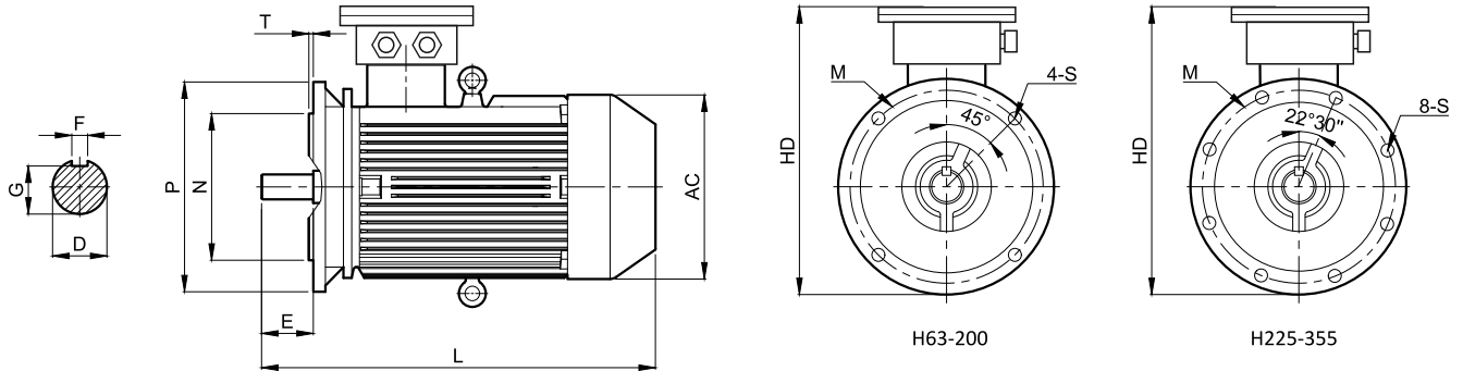
Mounting and overall dimensions Frame without feet, end-shield with flange (B5)
