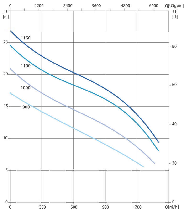
Performance Curves accor. to UNI 9906
