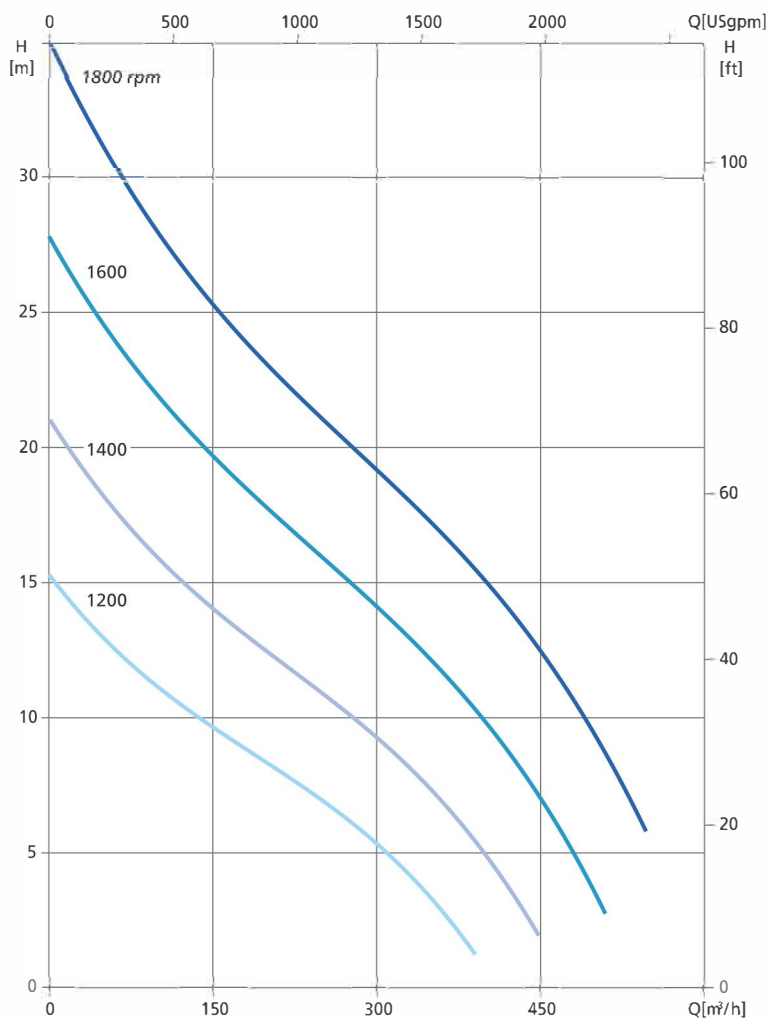
Performance Curves accor. to UNI 9906
